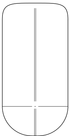
Elbow Narrow W: 100mm H: 200mm D: 95mm
