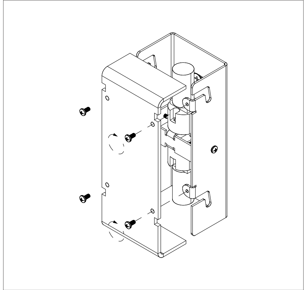
Mount the LED diffuser to the LED assembly with the previously removed machined screws
